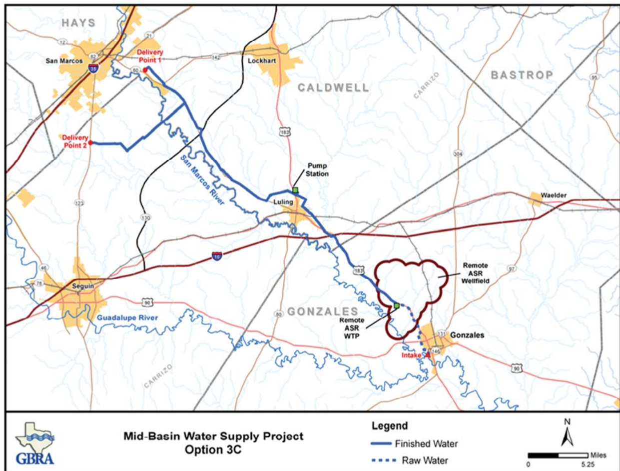
Figure 5.2.33-1 GBRA MBWSP – Surface Water with ASR Conceptual Layout
