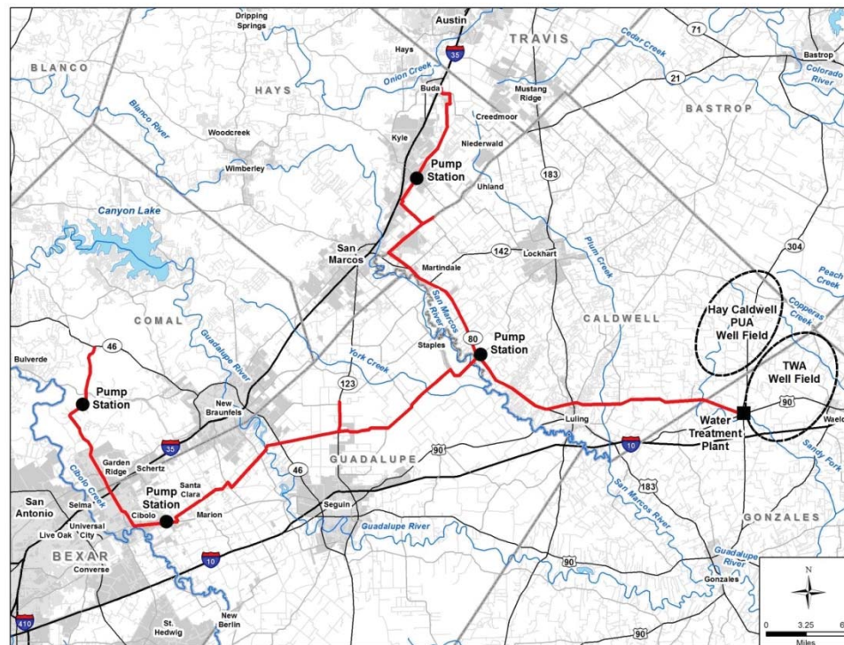
Figure 5.2.28-1 HCPUA / TWA Joint Project Conceptual Layout
