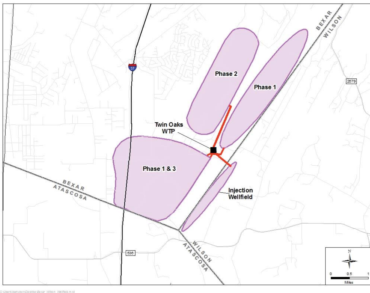
Figure 5.2.19-1 Brackish Wilcox Groundwater Desalination Project for SAWS
