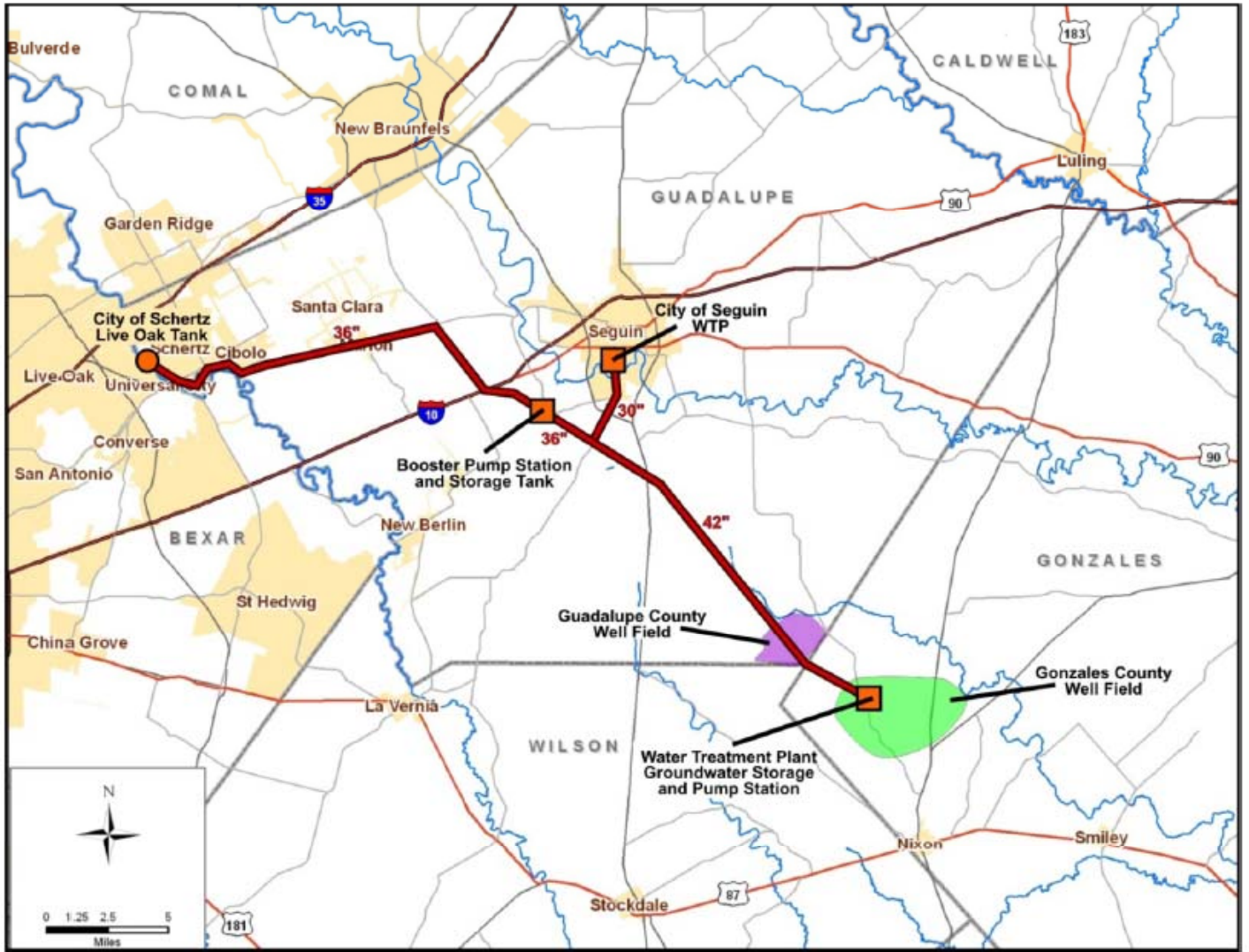
Figure 4C.19-1. Schertz-Seguin Water Supply Project
